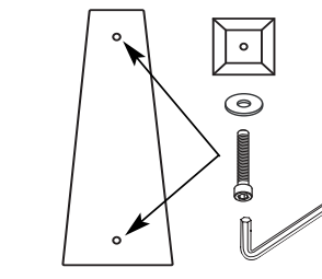
HTS104 Connecting Wedge
